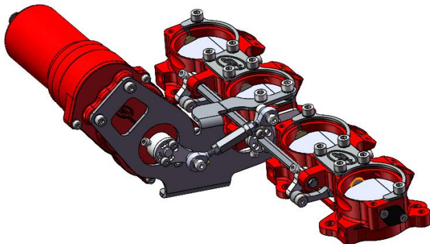
MOUNT 'C' 45 DEGREES LEFT PART No. 102-106-00080
